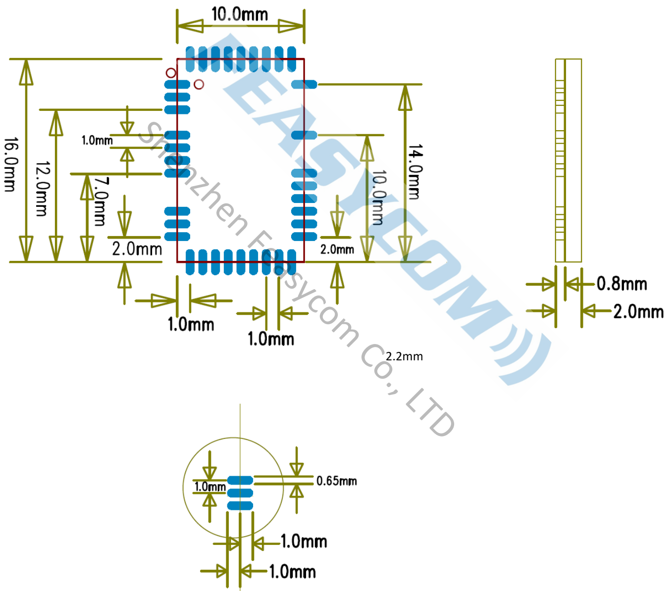
Figure 11: FSC-BT615V footprint
