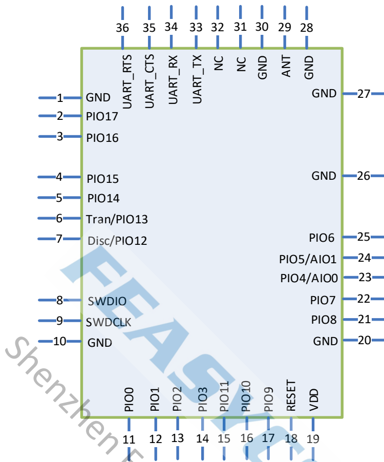
Figure 3: FSC-BT615V PIN Diagram(Top View)
