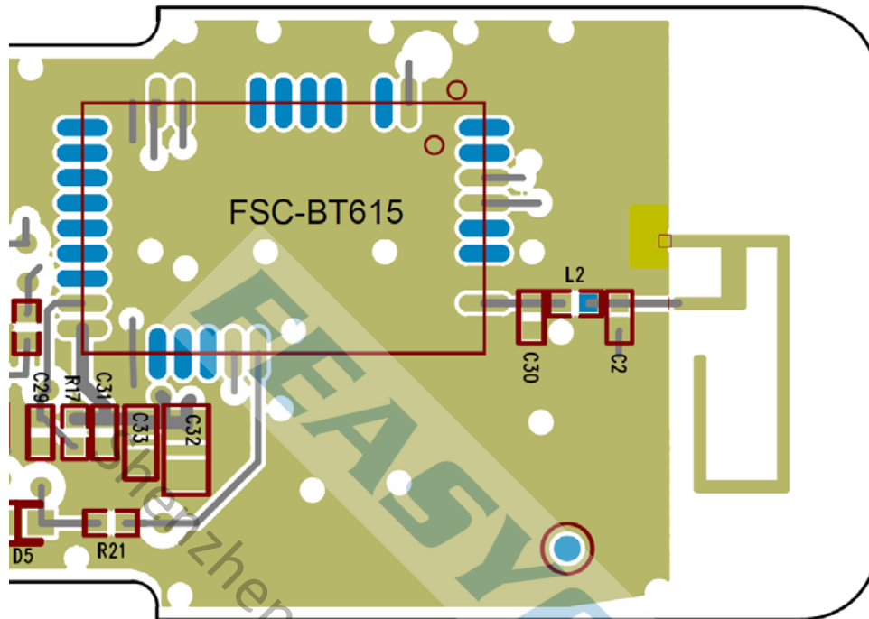
Figure 12: Host PCB-Top View
