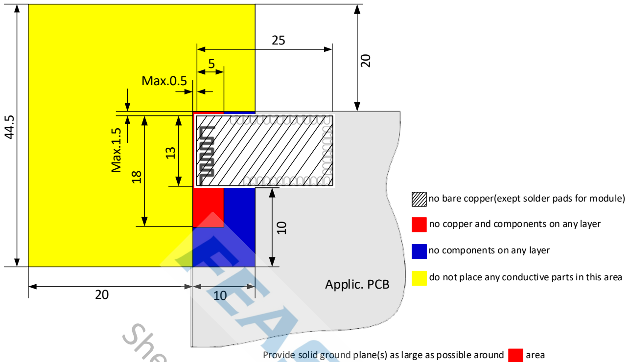
Figure 13: FSC-BT615V Restricted Area (Unit: mm)
